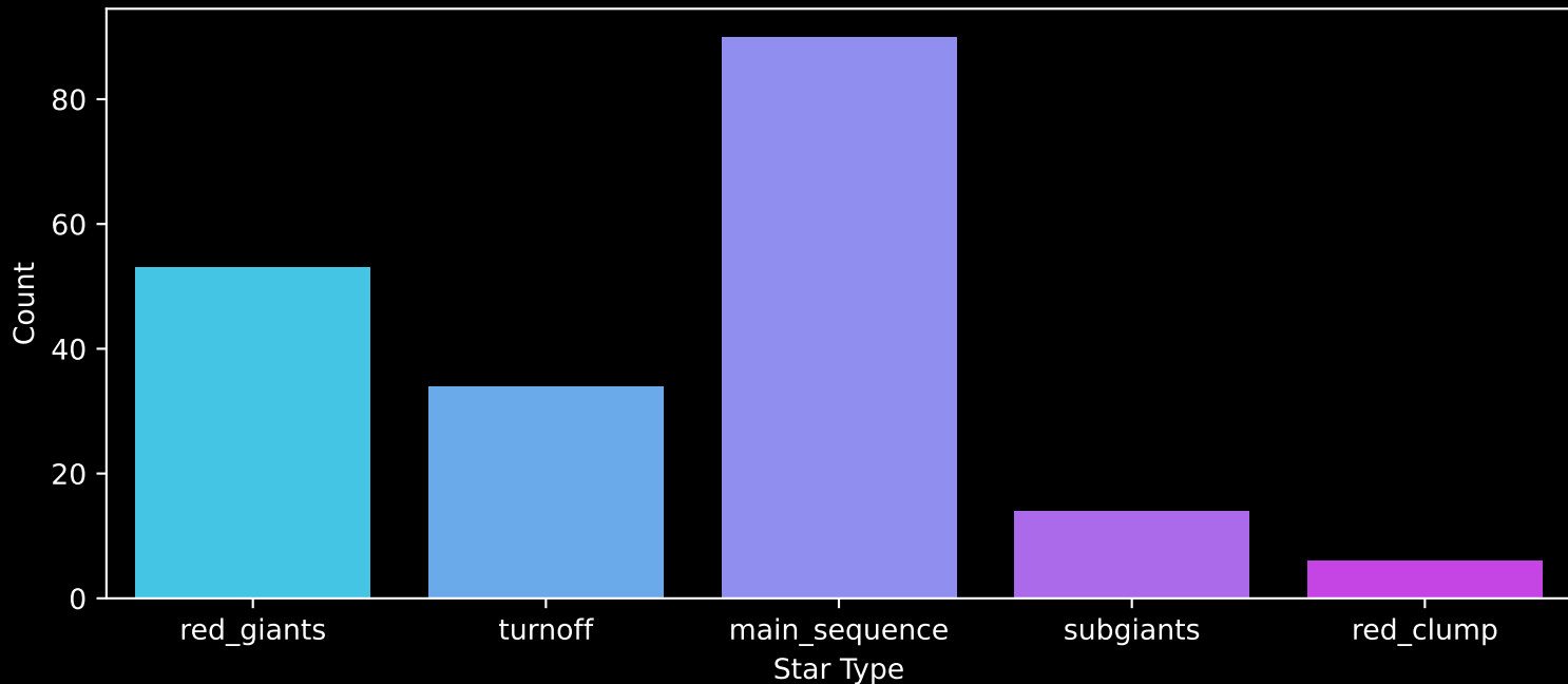
APOGEE DR17 Field: [244+45_MGA] Count plot of Star Type
