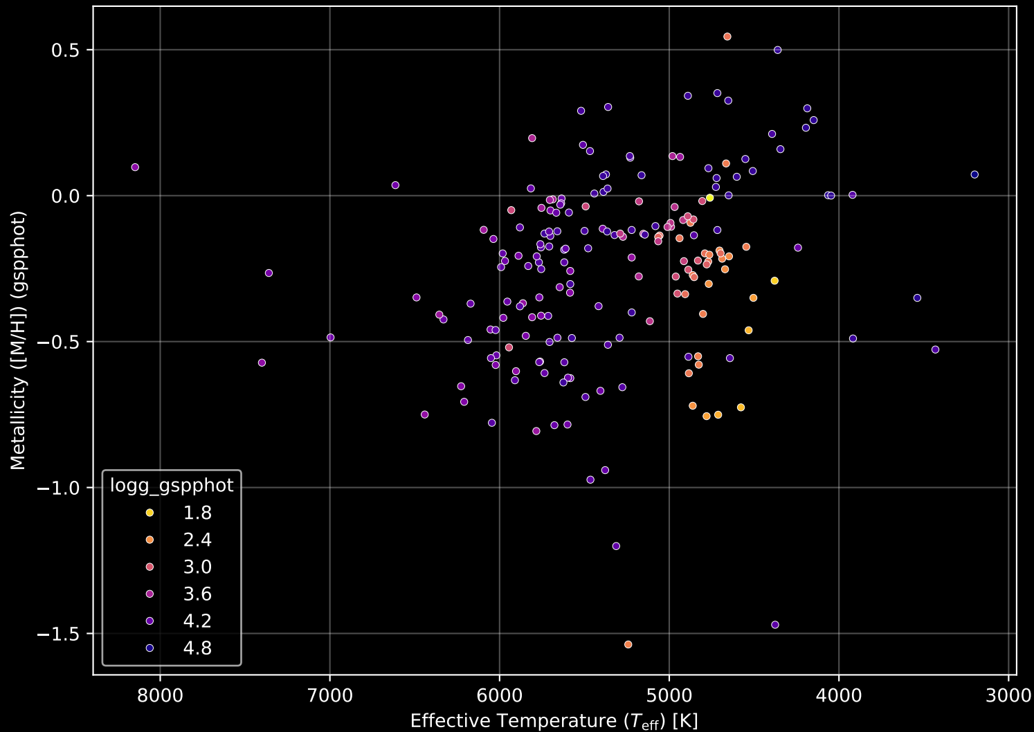
APOGEE DR17 Field: [244+45_MGA] Stellar Population Parameters (n= 197)
