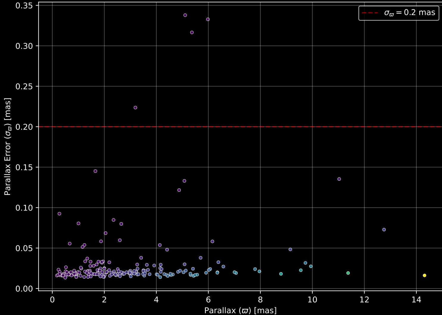
APOGEE DR17 Field: [244+45_MGA] Parallax Quality (n= 197)
