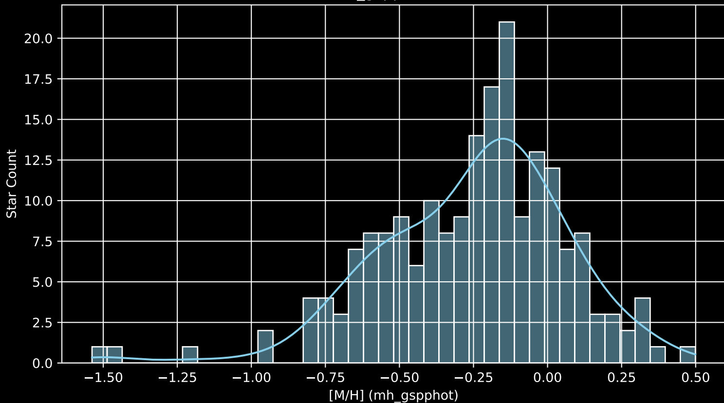
APOGEE DR17 Field: [244+45_MGA [M/H] (mh_gspphot) (n= 196)
