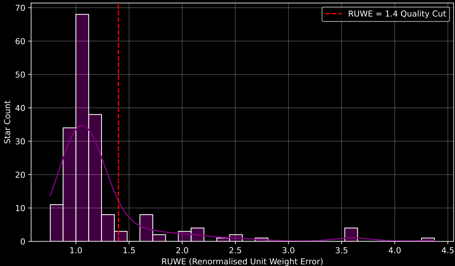
GAPOGEE DR17 Field [244+45_MGA] RUWE Distribution (n= 188)
