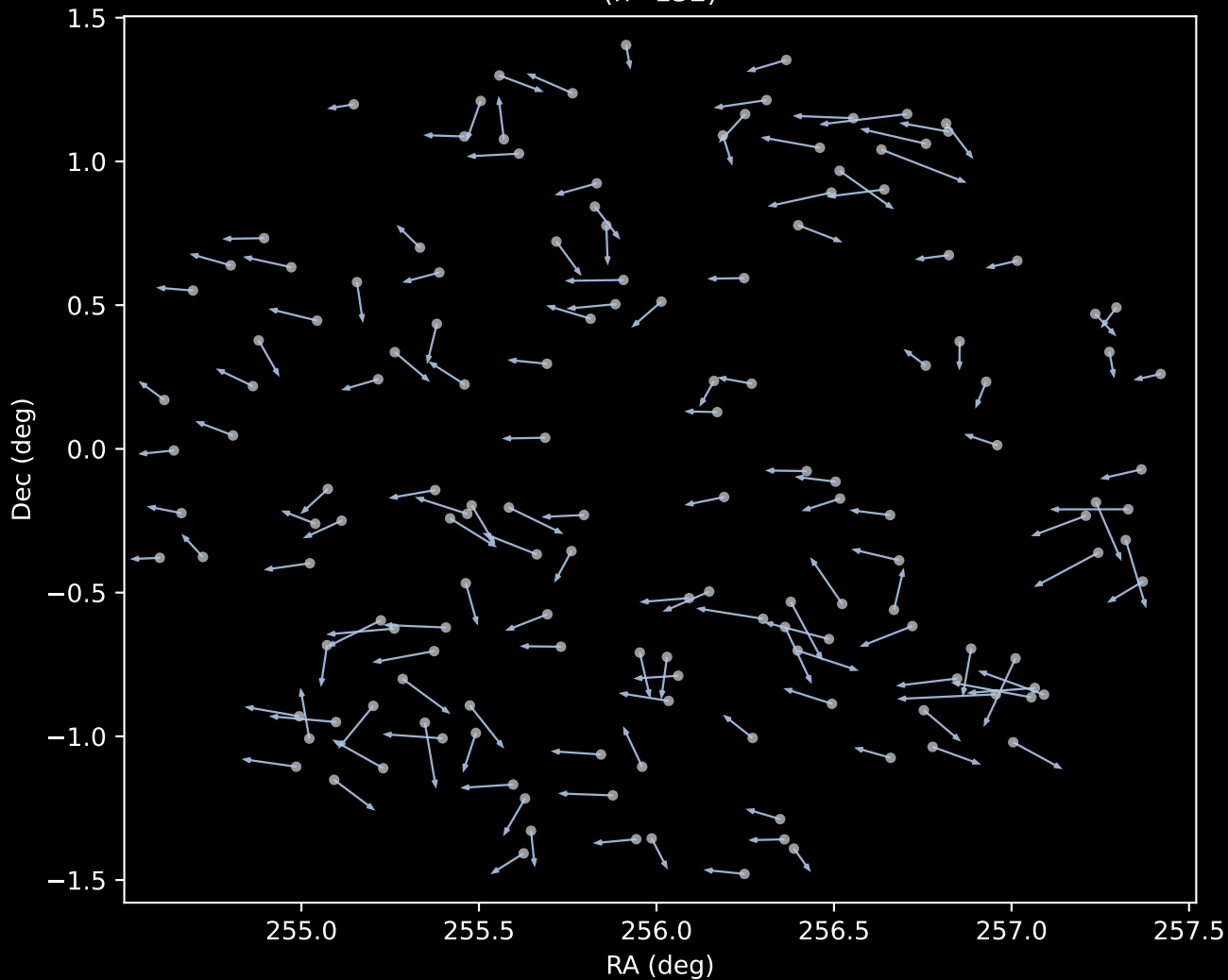
APOGEE DR17 Cluster 1 Proper Motion Vectors (n=152)
