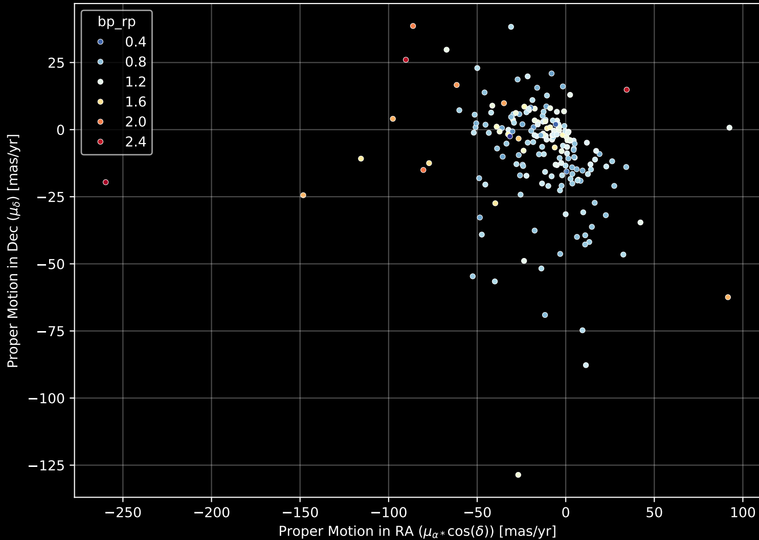
APOGEE DR17 Field: [244+45_MGA] Proper Motion Diagram (n= 197)
