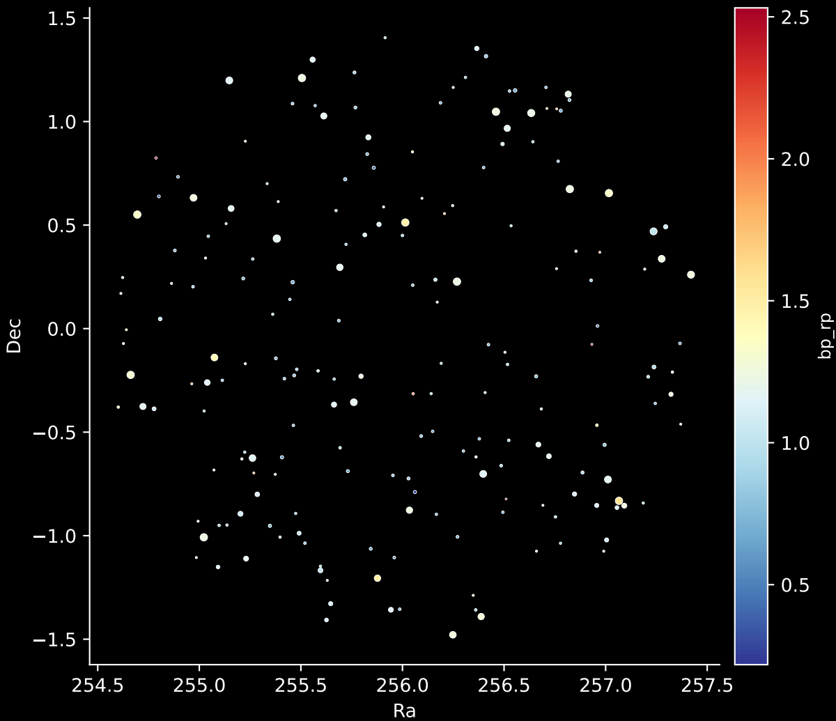
APOGEE DR17 Field: [244+45_MGA] Stars: 197
